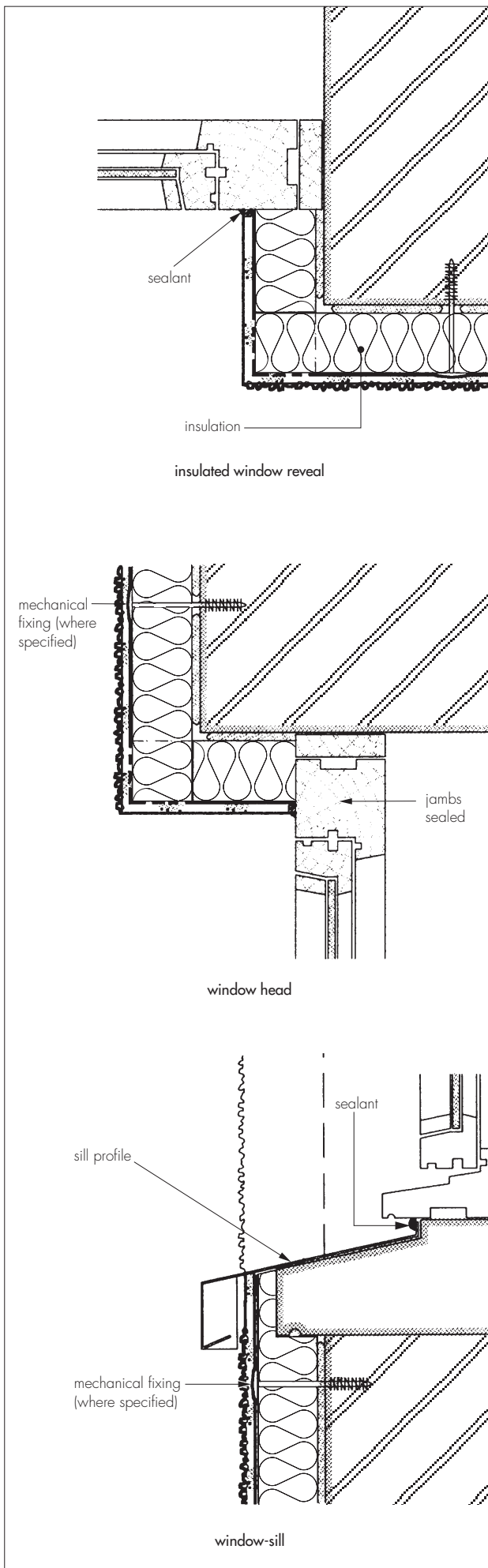
Figure 7 Window details
