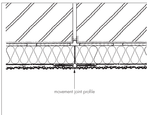
Figure 4 Vertical movement joint
