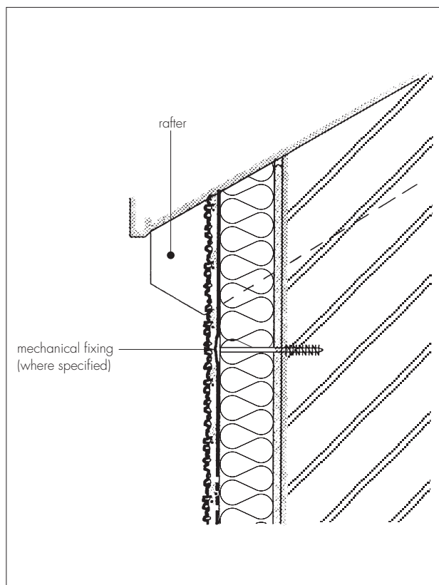
Figure 6 Eaves detail — pitched roof
