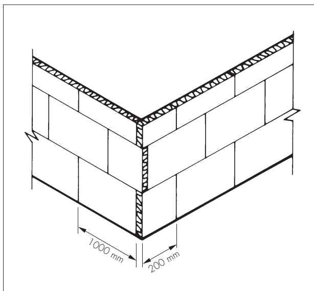
Figure 3 Arrangement of insulation boards
