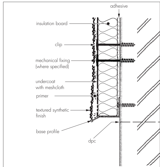
Figure 2 Typical section at base level
