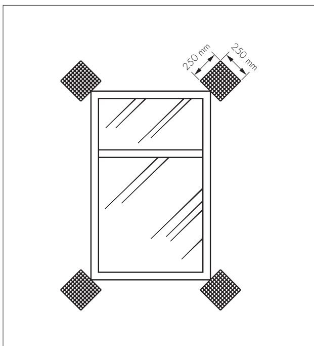
Figure 5 Additional reinforcement at openings
