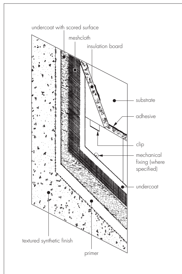
Figure 1 weber.therm XM (MFL) External Wall Insulation System
