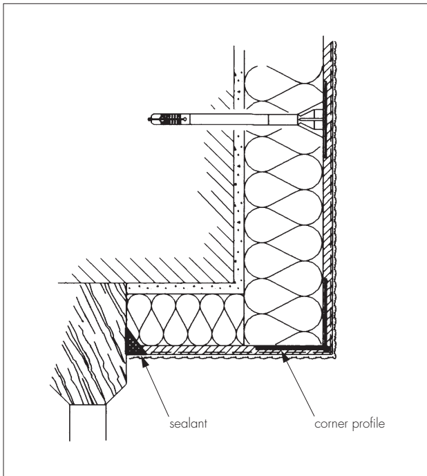
Figure 8 External corner detail
