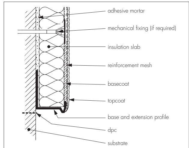
Figure 2 Typical section at base level
