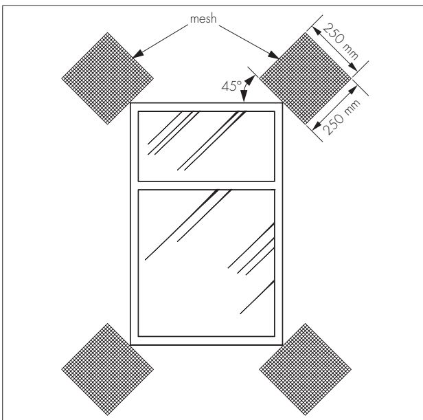
Figure 5 Additional reinforcement at openings
