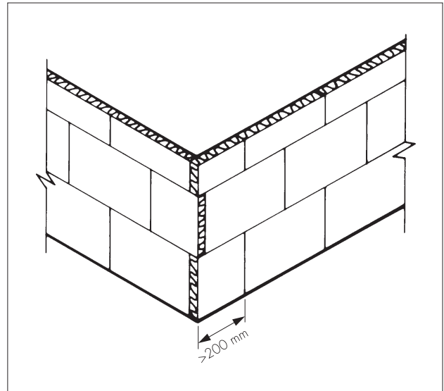
Figure 3 Arrangement of insulation boards
