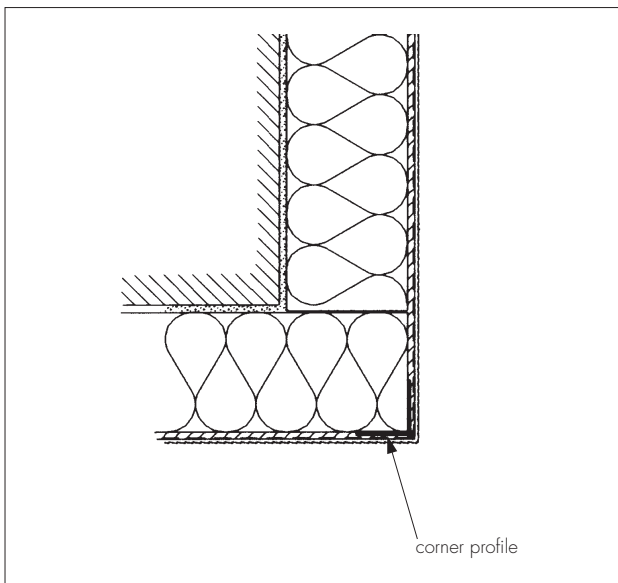
Figure 8 External corner detail
