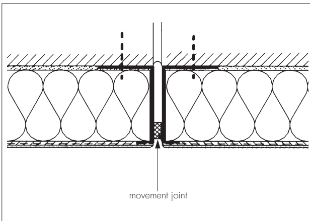
Figure 4 Vertical movement joint
