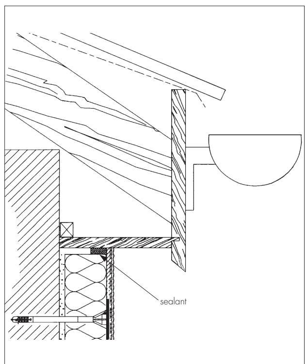
Figure 6 Roof eaves detail
