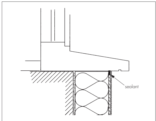
Figure 9 Window sill detail
