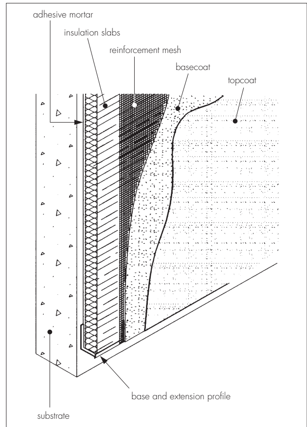
Figure 2 Typical section at base level
