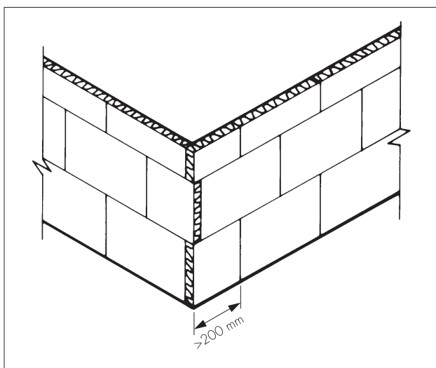
Figure 3 Arrangement of insulation boards
