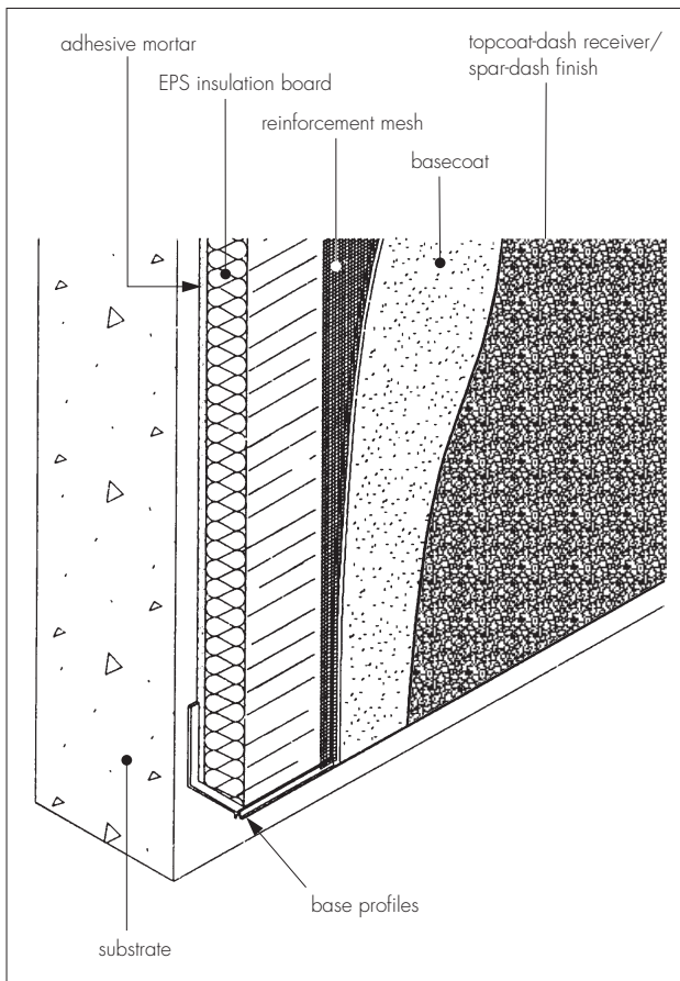
Figure 2 Typical section at base level
