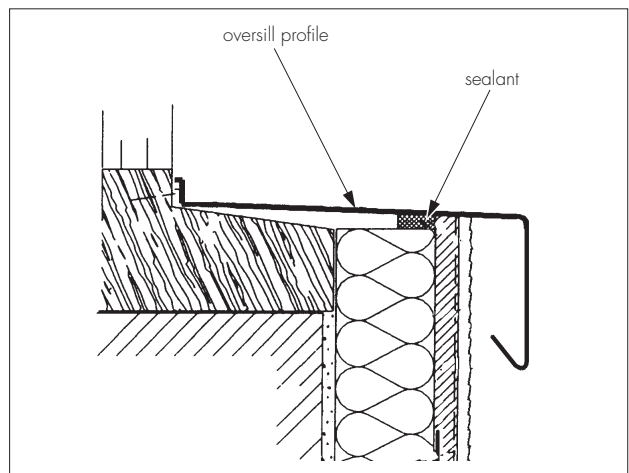
Figure 9 Window sill detail
