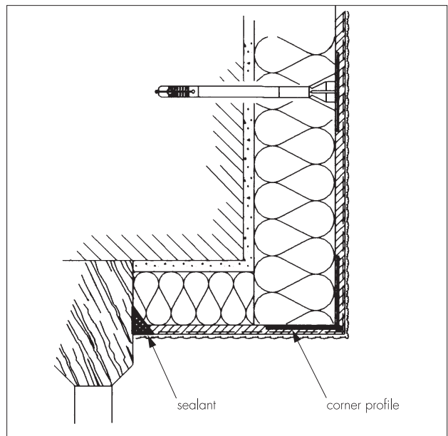
Figure 8 External corner detail
