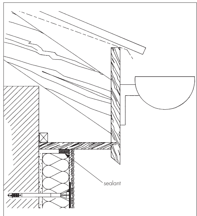
Figure 6 Roof eaves detail
