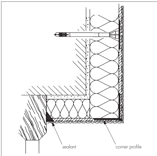
Figure 8 External corner detail
