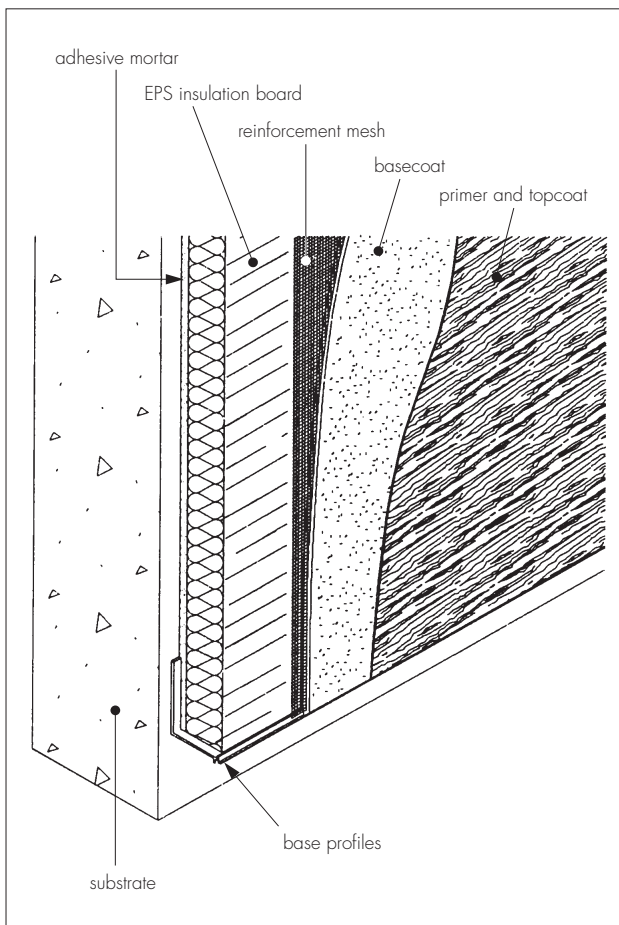
Figure 1 The Alsecco AWK2 External Wall Insulation System
